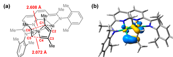
Figure 5. DFT calculations (M06/6-31G(d,p) level of theory) addressing the selectivity of alkyne addition to the bound butadienyl ligand. Propyne was used as a model substrate and i -Pr substituents on the catalyst were truncated to Me substituents. (a) The lowest-energy transition structure corresponding to the [4 + 2]-cycloaddition of the bound alkyne and butadienyl ligands. Distances for the two forming C–C bonds are shown in red. (b) The HOMO–1 for the metallacycle intermediate.
