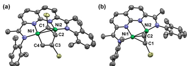
Figure 4. Solid-state structures of (a) 12 and (b) 13 (ellipsoids at 50% probability). i -Pr groups on the NDI ligand and substituents on silicon are truncated for clarity. Selected bond distances for 12 (Å): Ni1–Ni2, 2.4814(6); Ni1–C1, 1.942(2); Ni1–C4, 1.868(2); Ni2–C1, 1.875(2); Ni2–C2, 2.042(2); C1–C2, 1.416(4); C2–C3, 1.482(3); C3–C4, 1.350(3). Selected bond distances for 13 (Å): Ni1–Ni2, 2.3140(6); Ni1–C1, 2.023(3); Ni1–C2, 1.911(3); Ni2–C1, 2.015(2); Ni2–C2, 1.904(2); C1–C2, 1.301(4).
