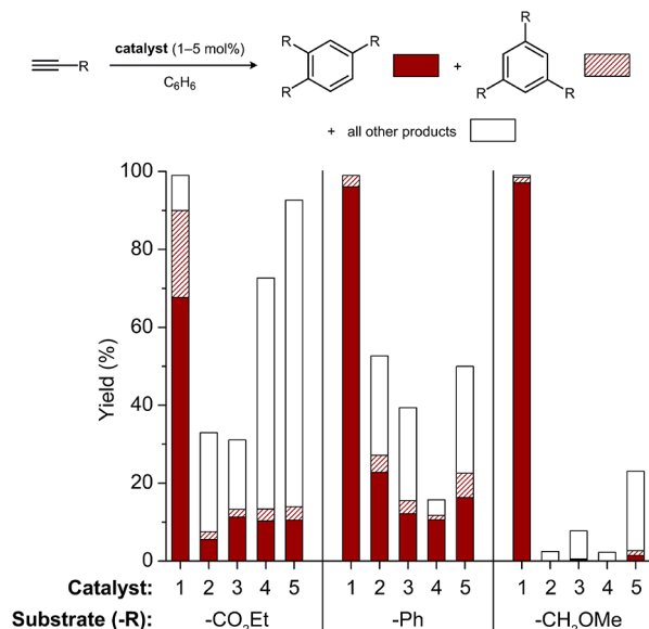
Figure 2. A comparison of catalytic activity for the cyclotrimerization of ethyl propiolate, phenylacetylene, and methyl propargyl ether. Data for catalysts 1–4 and Ni(COD) 2 (5) are shown. Reaction conditions for ethyl propiolate and methyl propargyl ether: 22 °C, 11 min, 1 mol % catalyst. Reaction conditions for phenylacetylene: 60 °C, 40 min, 5 mol % catalyst. Yields and conversions were averaged over two runs and determined by GC-FID analysis. The total heights of the bars are the total conversion of starting material. The product fraction corresponding to the 1,2,4-isomer (solid red), 1,3,5-isomer (dashed red), and all other products (white) are plotted.
